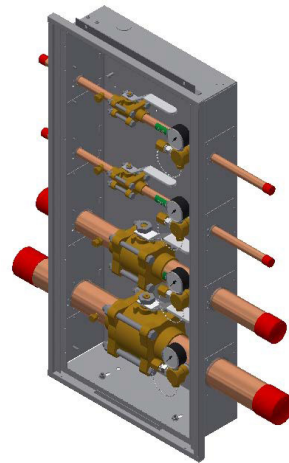
EV Series Zone Valve Box
