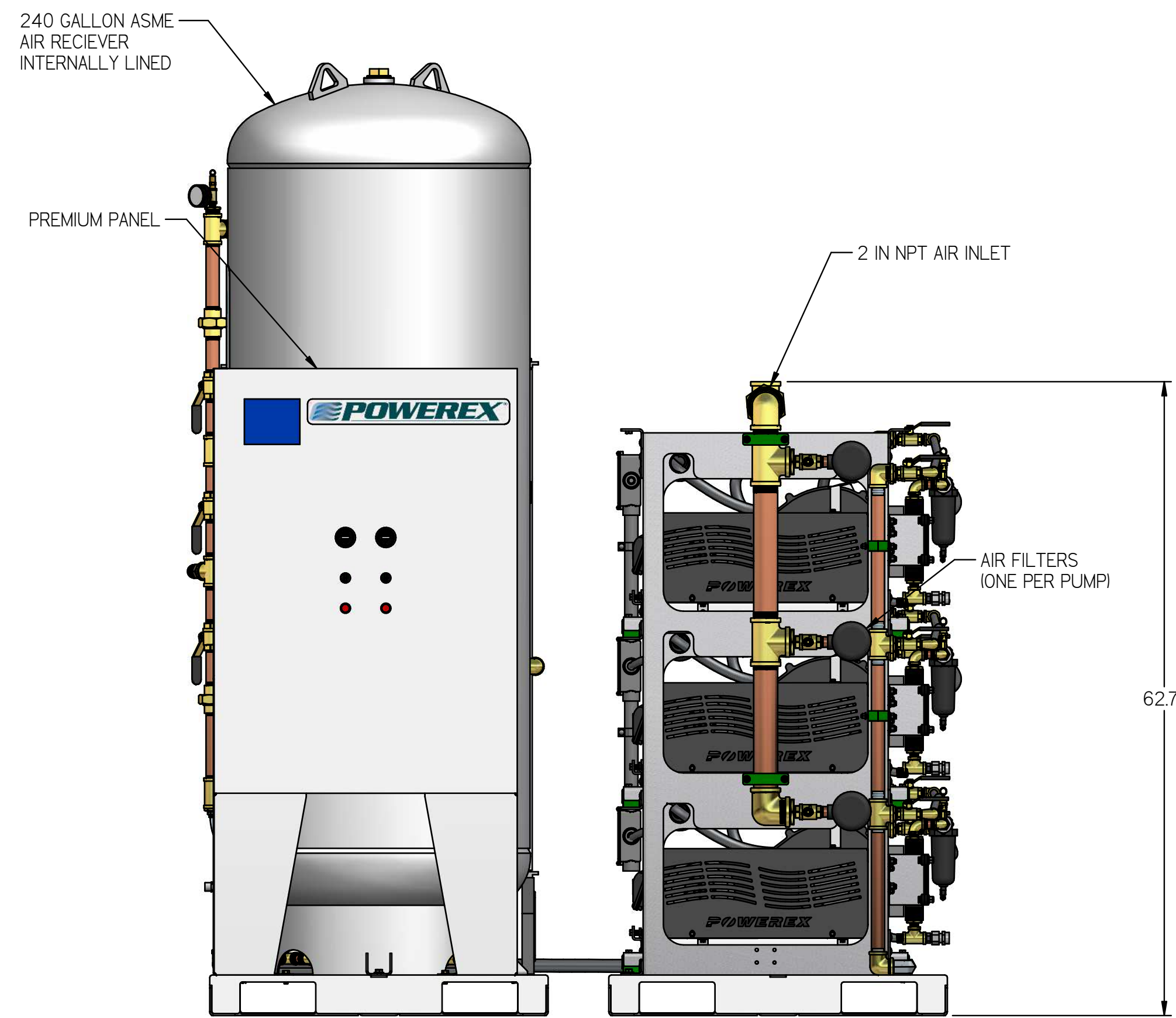
FRONT VIEW
