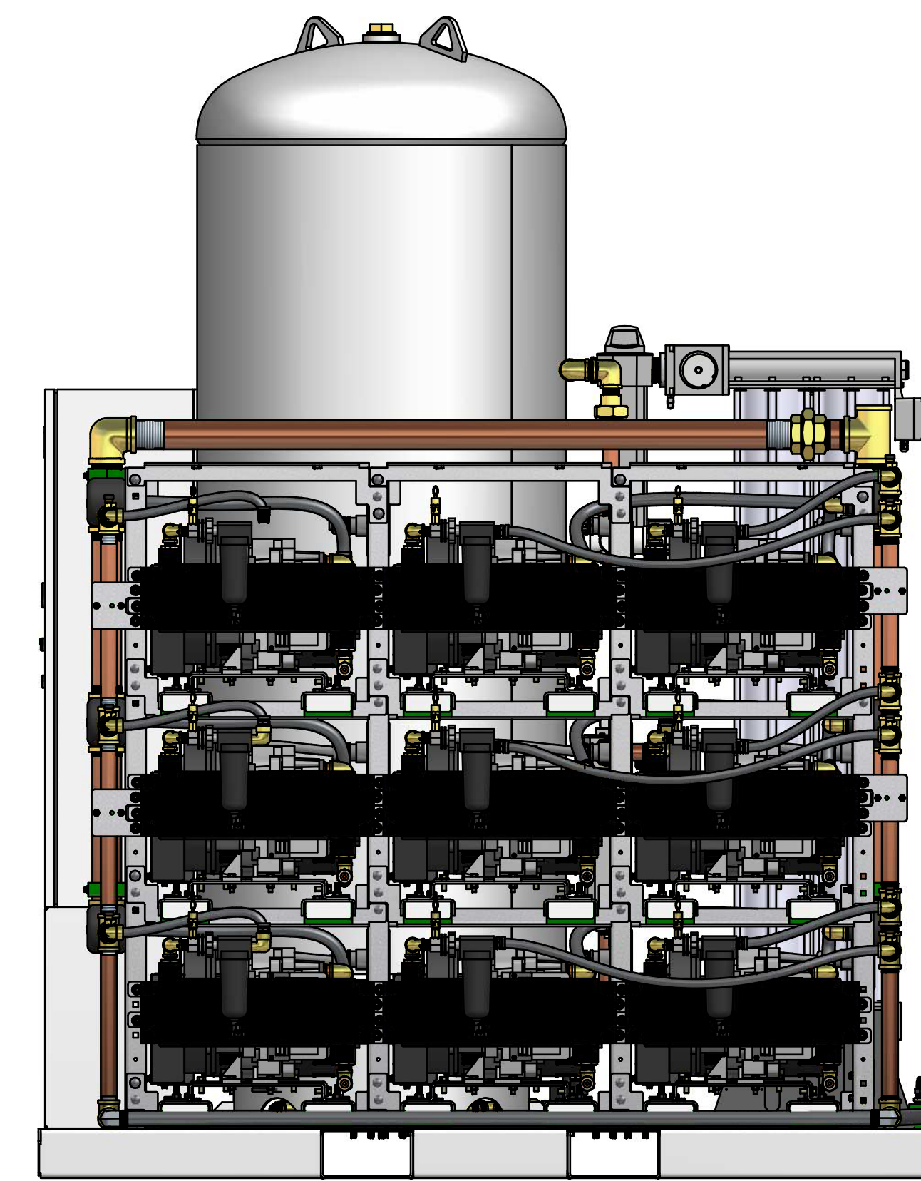
RIGHT VIEW
