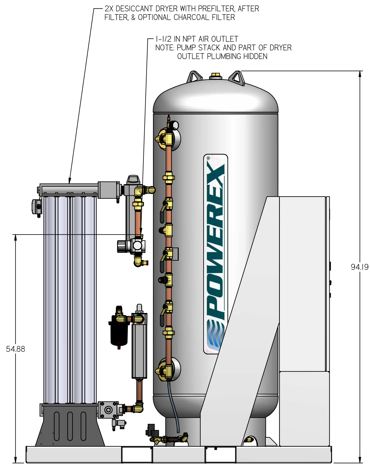
LEFT VIEW
