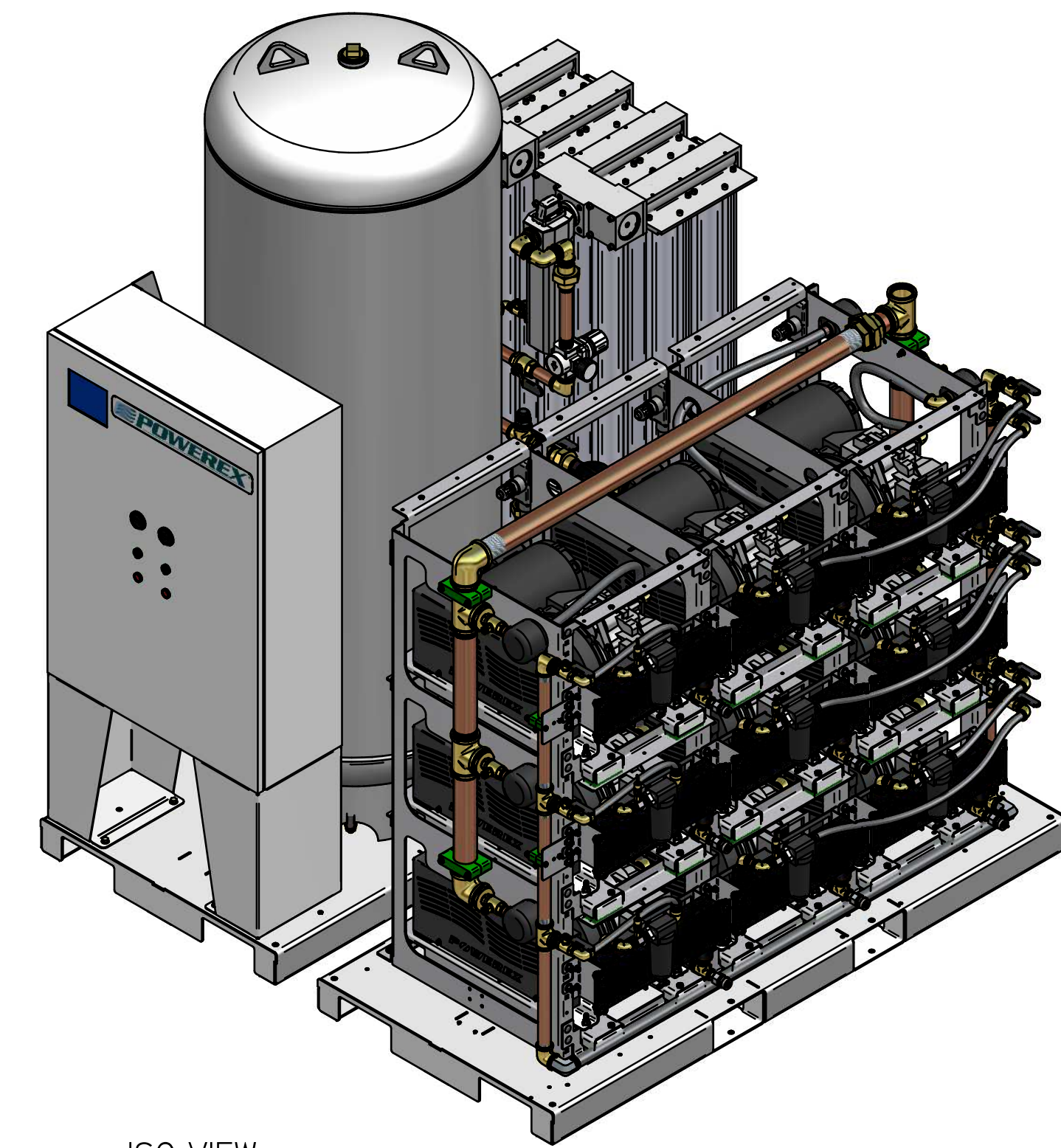
ISO VIEW
