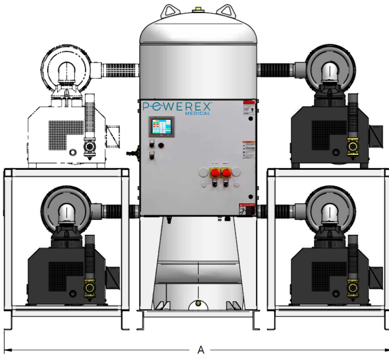
Claw Vacuum Package Specification
