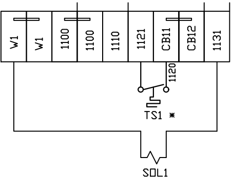
PLEX #1 CONNECTIONS
